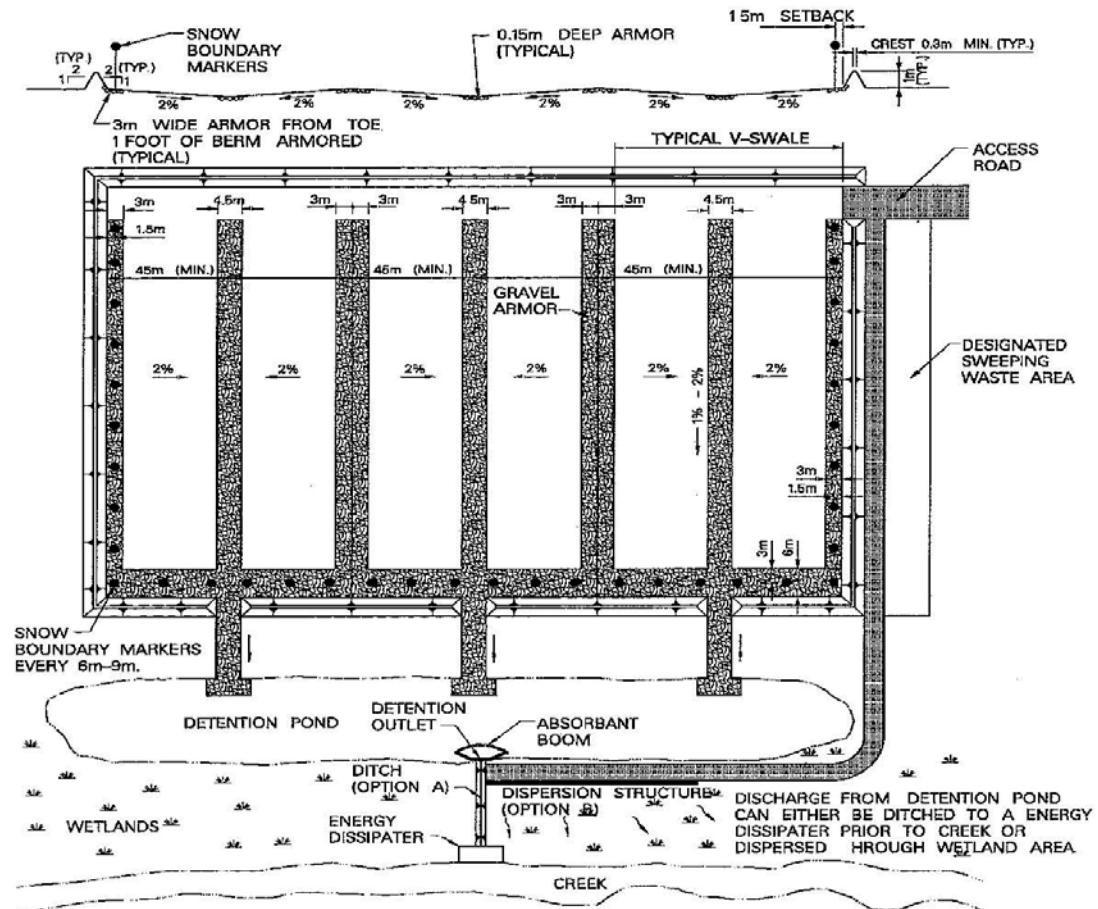
Figure 8.2-1: Multiple V-Swale Snow Site Design Concept
